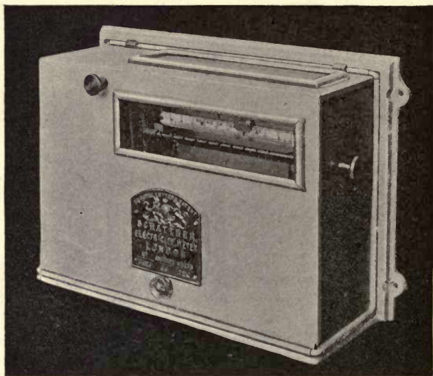
Fig. 230.—Schattner Standard Meter (Cover in position)
